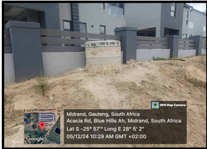
Figure 13: The Installed Manhole
